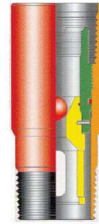
Liner Hanger
