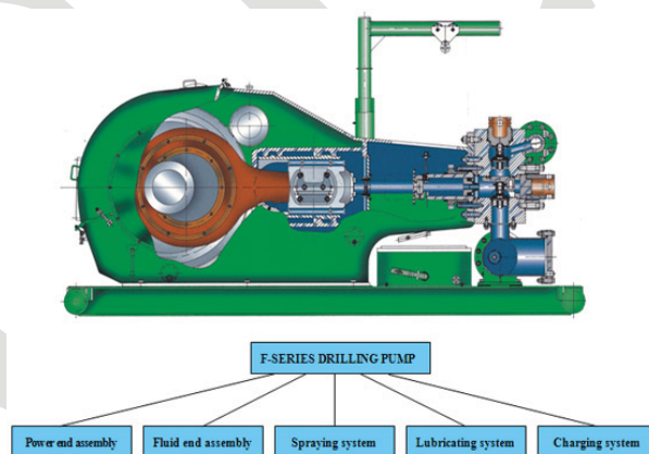
F Series Mud Pump
