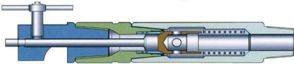
Inside BOP
